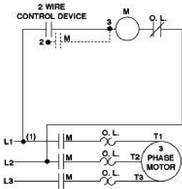
ELEMENTARY DIAGRAM OF STARTER (2-WIRE CONTROL)
