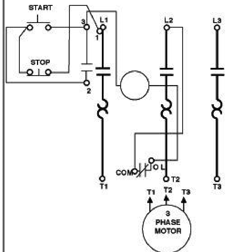
WIRING DIAGRAM OF STARTER (3-WIRE CONTROL)
