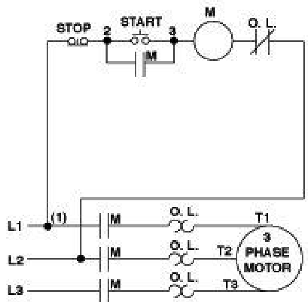
ELEMENTARY DIAGRAM OF STARTER (3-WIRE CONTROL)
