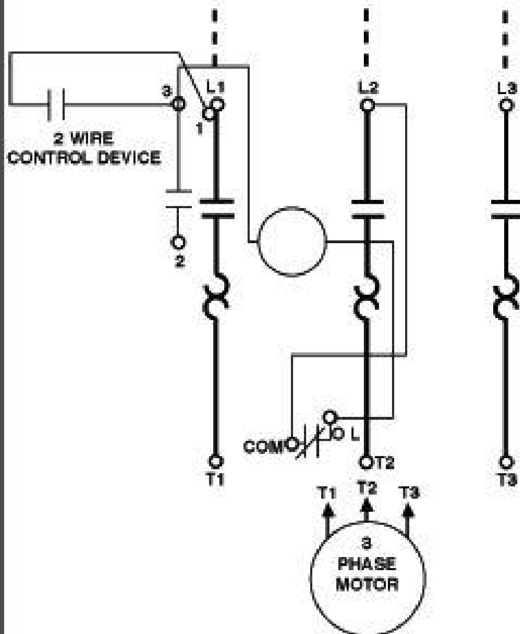
WIRING DIAGRAM OF STARTER (2-WIRE CONTROL)
